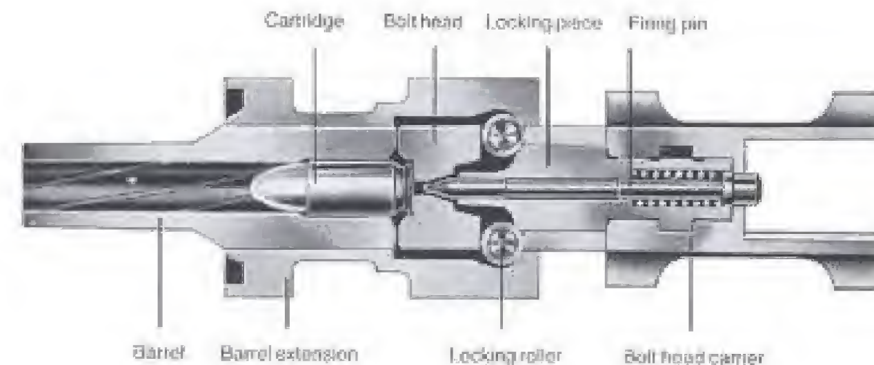
Fig. 27 Bolt in locked position
